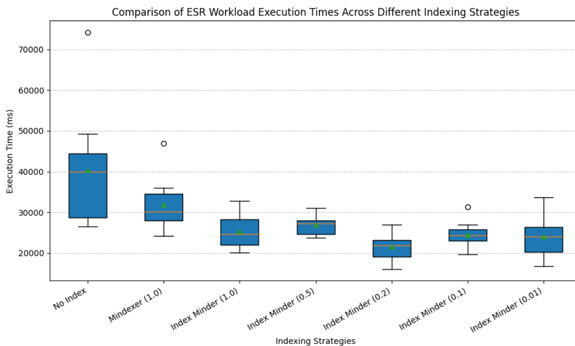
FIGURE 5.6: Performance Evaluation (ESR Workload)
